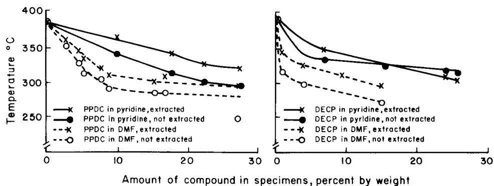
FIG. 3. Temperature at maximum rate of pyrolysis of wood specimens reacted with increasing amounts of phenylphosphonic dichloride (PPDC) or diethylchlorophosphate (DECP). (ML86 5406)
