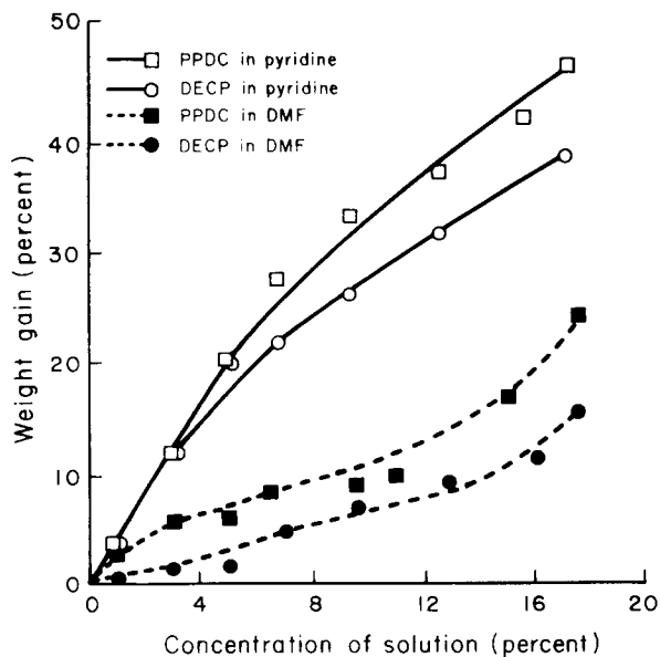
FIG. 1. Weight gain of wood specimens reacted with phenylphosphonic dichloride (PPDC) or diethylchlorophosphate (DECP) in pyridine or dimethylformamide (DMF). (ML86 5404)
