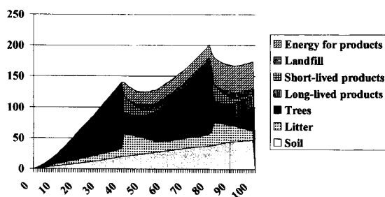
FIG. 2. Cumulative changes in carbon stocks with afforestation and subsequent harvest after 40 year rotation. Source: Marland and Schlamadinger 1999.
