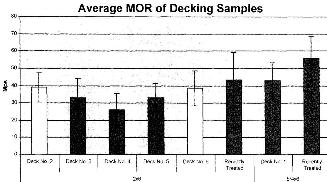
FIG. 6. Mean and range of the MOR data from the removed decking and recently treated sample sets.
