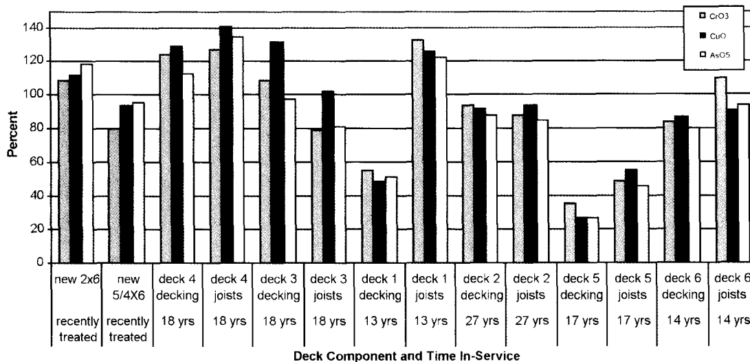
FIG. 2. Ratio of the current chemical retention level to the level indicated by the AWPA stamp or tag located on the test specimens.
