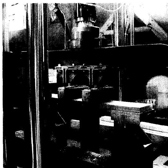
FIG. 1. MTS with test specimen loaded flat-wise in third point loading system.
