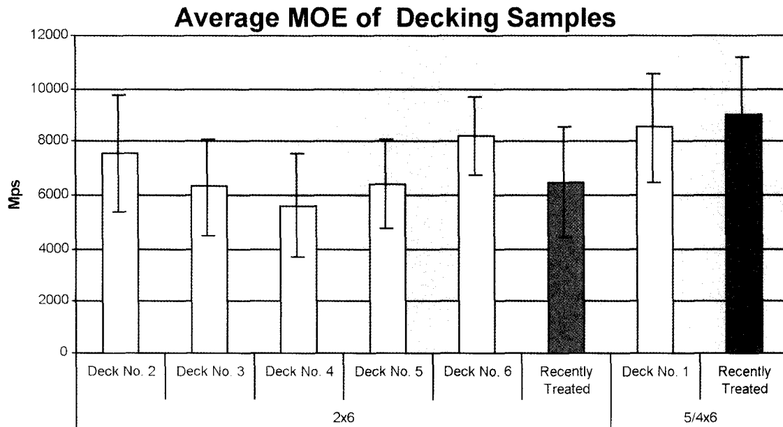
FIG. 5. Mean and range of the MOE data from the removed decking and recently treated samples.
