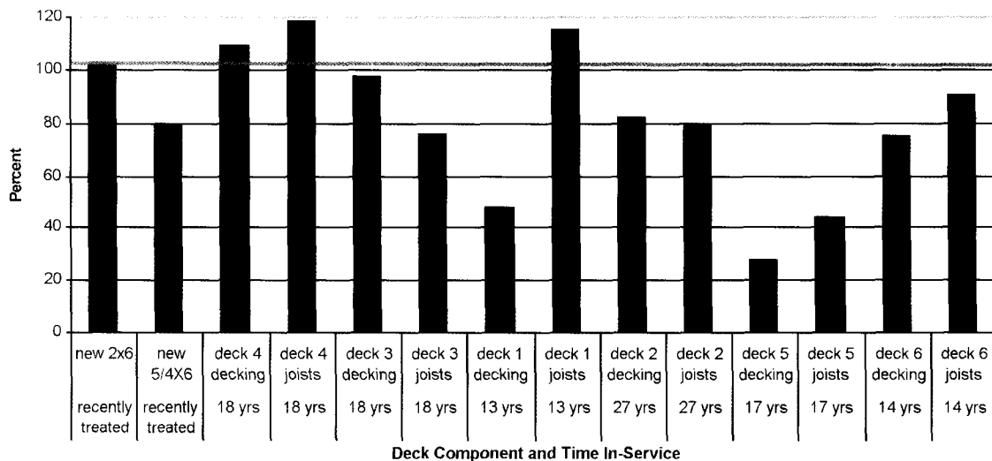
FIG. 3. Ratio of actual chemical retention to required minimum chemical retention by AWWA of chemical assay samples.
