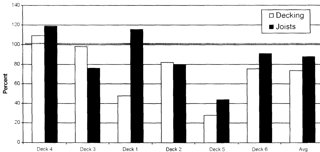
FIG. 4. Comparison of the ratio of current retention levels to that required at treatment of the recovered decking and joists of the discarded decks.
