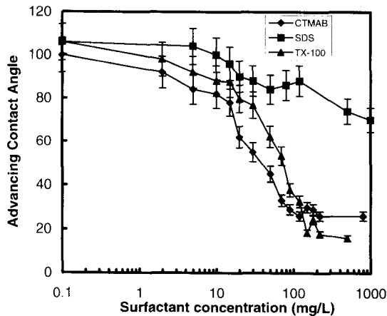
FIG. 9. Advancing contact angle of 0.6% AKD sized fibers in different surfactant solutions as a function of surfactant concentration at neutral pH and room temperature.
