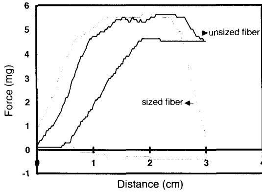
FIG. 5. The traces of dynamic wetting force of 0.2% AKD sized and unsized bleached southern pine fibers in water.
