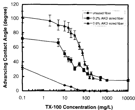
FIG. 7. Advancing contact angle of unsized, 0.2% AKD sized, and 0.6% sized bleached southern pine fibers as a function of TX-100 concentration.
