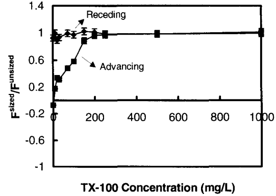
FIG. 6. The ratio of the dynamic wetting forces measured from unsized and 0.6% AKD sized southern pine fibers against surfactant concentration.
