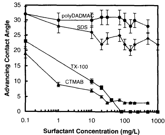
FIG. 8. Advancing contact angle of unsized bleached southern pine fibers in different surfactant solutions as a function of surfactant concentration at neutral pH and room temperature.
