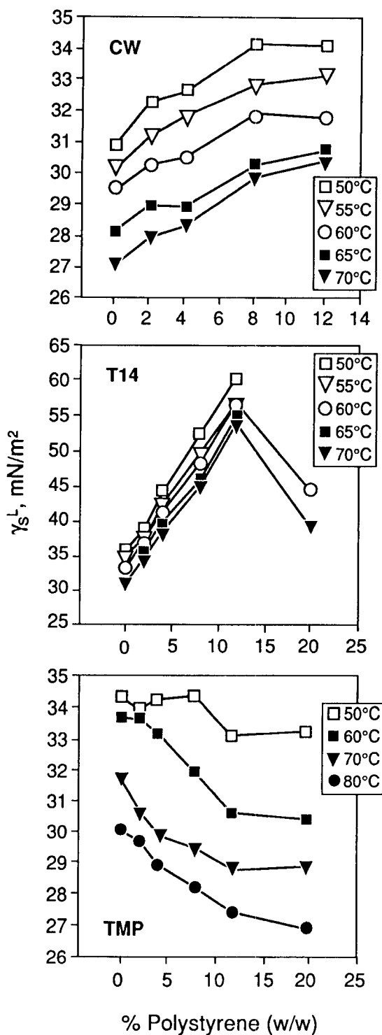
FIG. 6. London component of the surface free energy for CW, T14, and TMP substrates as a function of PS loading.
