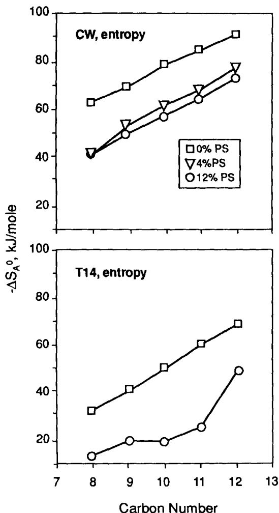
FIG. 5. Entropy as a function of probe carbon number for PS-coated CW and T14 substrates.
