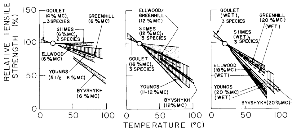
FIG. 15. Effect of temperature on tensile strength perpendicular-to-the-grain. 100% at 20 C. A: 4-6% MC. B: 11-16% MC. C: \geq 18% MC.
