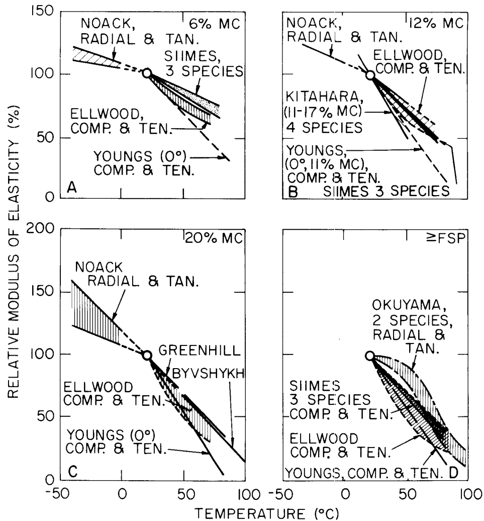
FIG. 4. Effect of temperature on modulus of elasticity perpendicular-to-the-grain. 100% at 20 C. A: ~6% MC. B: ~12% MC. C: ~20% MC. D: \geq FSP.
