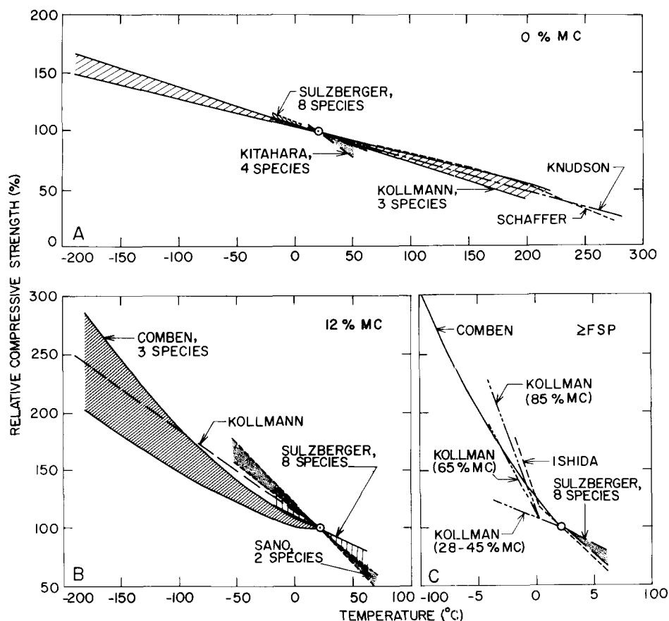
FIG. 11. Effect of temperature on compressive strength parallel-to-the-grain. 100% at 20 C. A: 0% MC. B: ~12% MC. C: \geq FSP.
