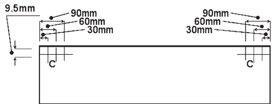
Figure 3. Face member with distances where the connectors (C = cam fastener) were placed in the first study.
