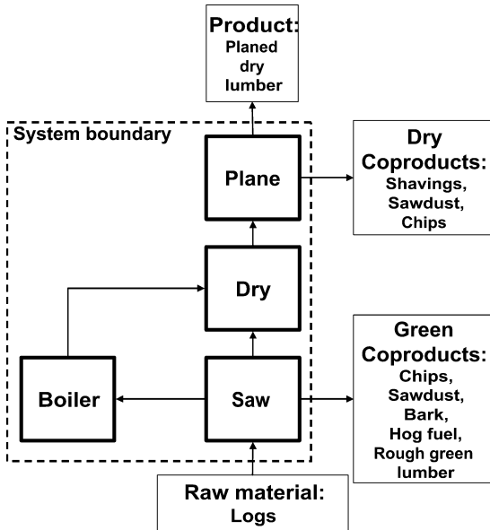
FIG. 1. Flow diagram for lumber production. Bold borders indicate the four unit processes. Dashed line indicates system boundary. Only wood materials are shown for clarity. Other materials and fuels also cross system boundary.
