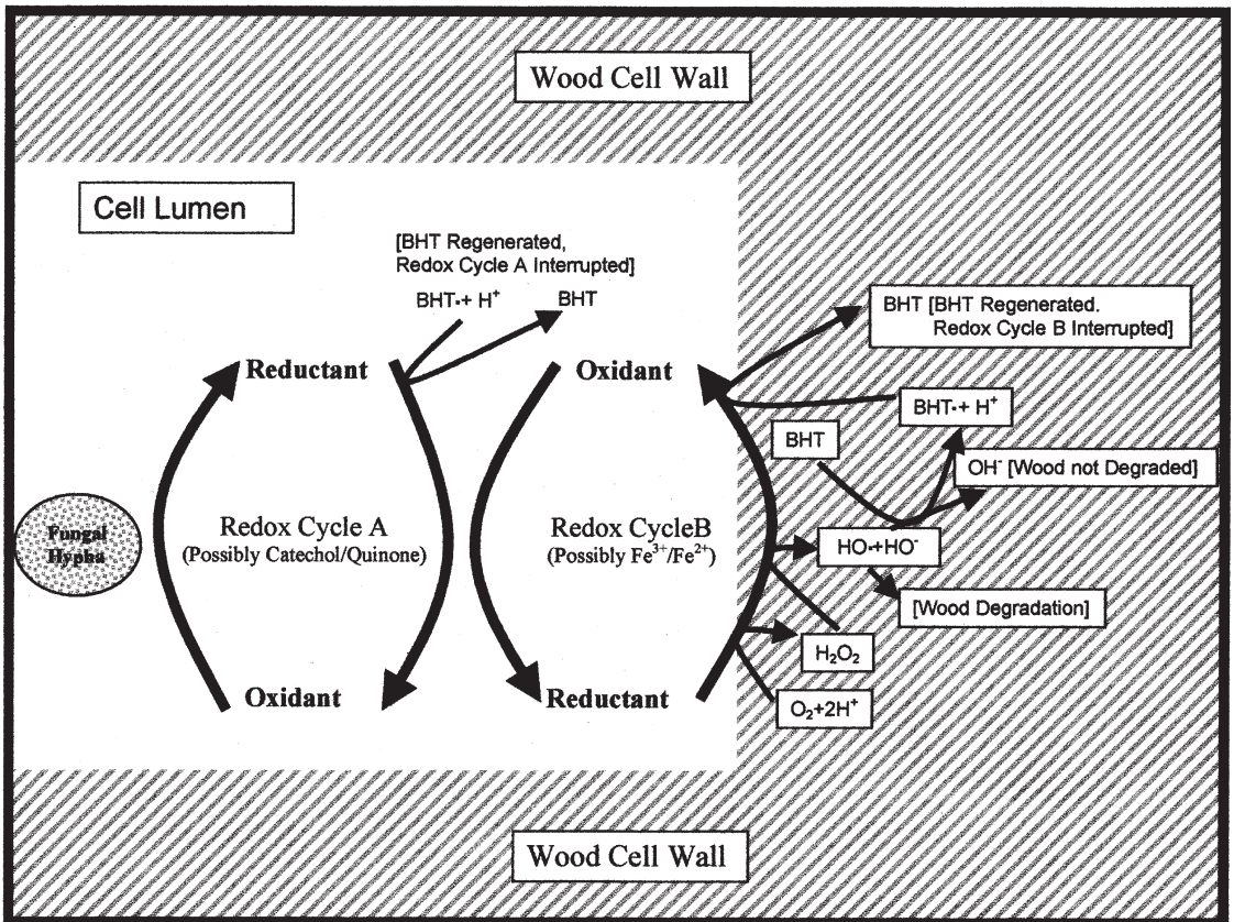
Fig. 1. Generalized hypothetical scheme of how brown-rot fungi could degrade wood with multiple interconnected redox cycles, and a proposed scheme for how BHT, or other free radical scavengers (antioxidants), might interfere with the fungal generated radical reagents which attack wood. In addition, we propose a possible mechanism by which the BHT radical, formed by scavenging a free radical, might be regenerated by the reductive portion of one or more of the fungal redox cycles.
