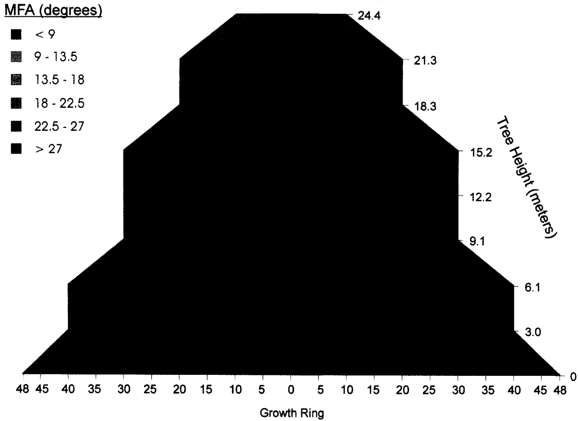
FIG. 8. Map of fiber microfibril angle shown as function of location within a tree.
