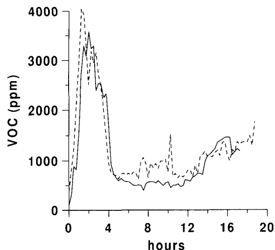
FIG. 1. Method 25A profiles collected from a commercial southern pine dry kiln in July 2000 (bold) and November 2000 (dashed).
