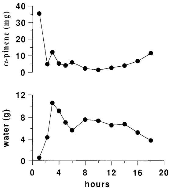
FIG. 2. \alpha -pinene and water profiles collected from the commercial dry kiln run in July 2000.
