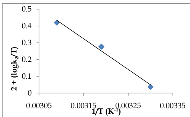
Fig 4: Eyring's Plot
