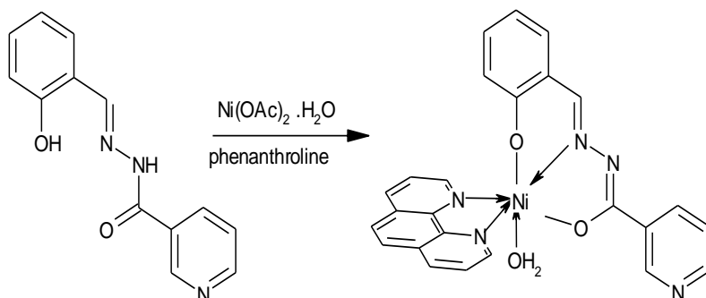
Fig. 1. Scheme of the synthesis of NiL^3phen
