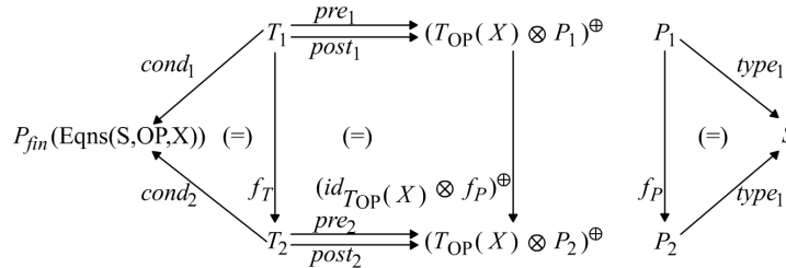
Figure 2: Condition for AHL-Net morphisms.
