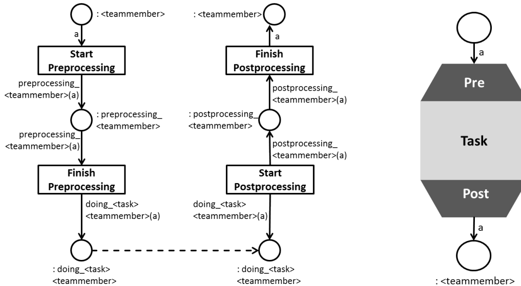
Figure 11: Left: The pattern of Places and Transitions used to represent a task. Right: A visual abbreviation for the pattern.
