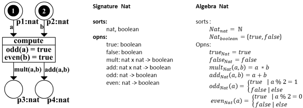
Figure 1: Example - AHL-Net(left), Signature (middle) and Algebra (right).
