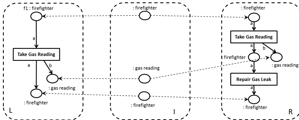
Figure 8: A transformation rule for inserting the task Repair Gas Leak after the task Take Gas Reading
