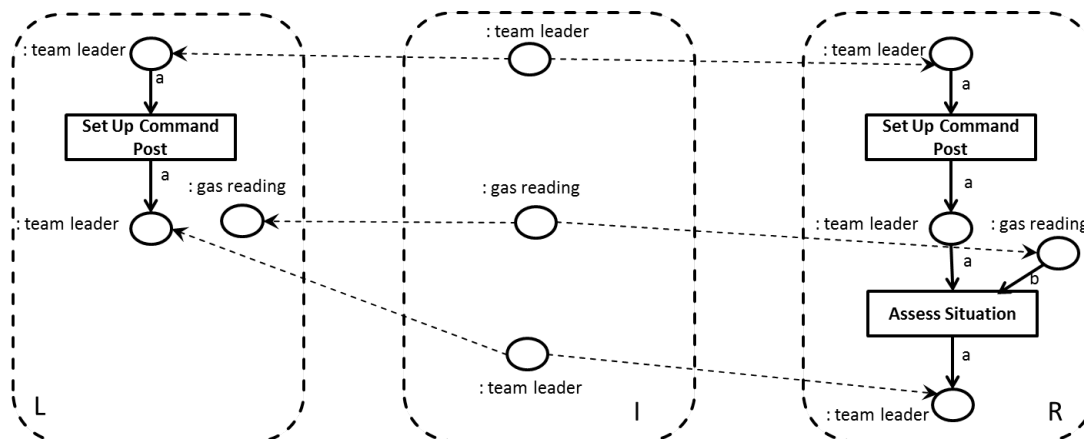
Figure 18: Insertion rule for the task Assess Situation .
