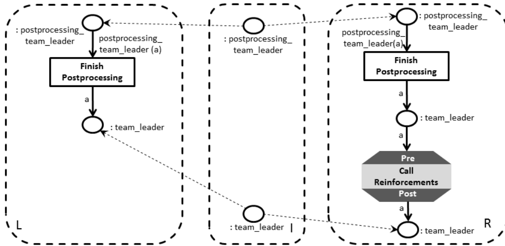
Figure 32: Insertion rule for the task Call Reinforcements .
