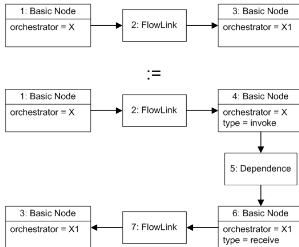
Figure 3: Rule AddDependence
