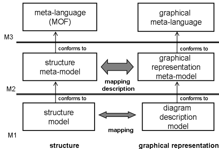
Figure 1: The meta-architecture of the approach
