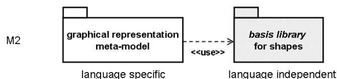
Figure 4: The graphical representation meta-model uses a language independent basis library
