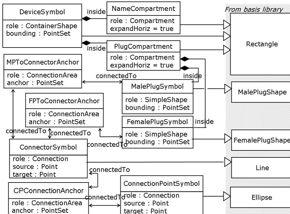
Figure 5: A subset of the graphical representation meta-model (M2) for the Service language
