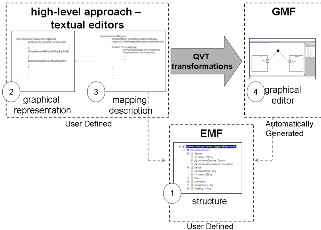
Figure 8: An overview of the implementation
