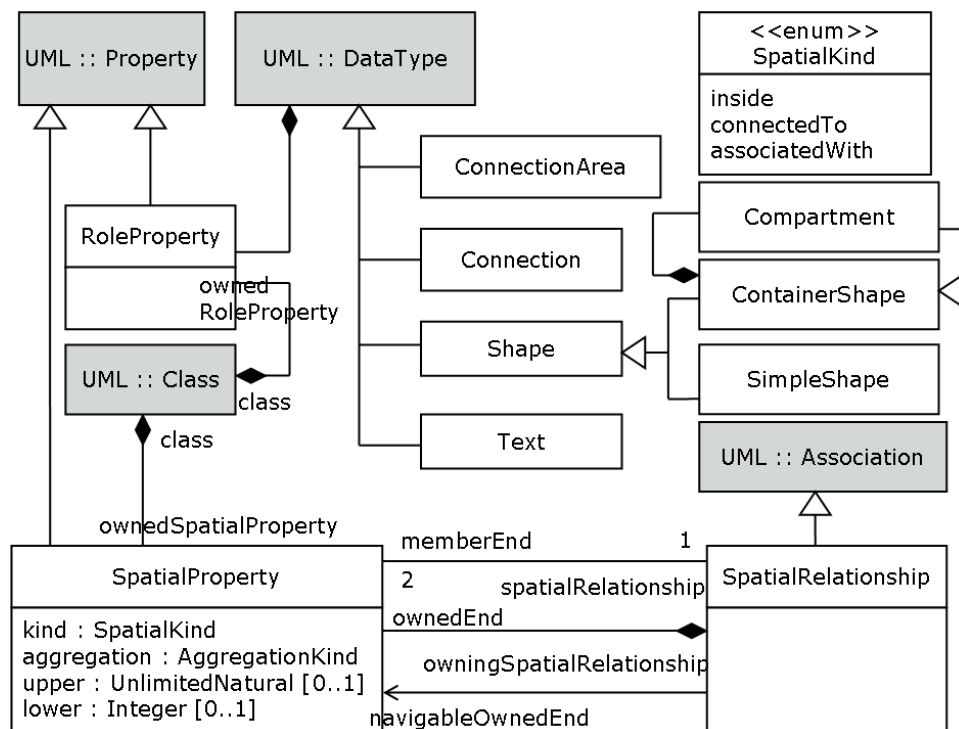
Figure 6: The meta-language (M3) for graphical representations
