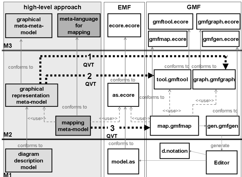
Figure 9: An overview of the high level approach (left-hand side) and its transformation to the GMF platform
