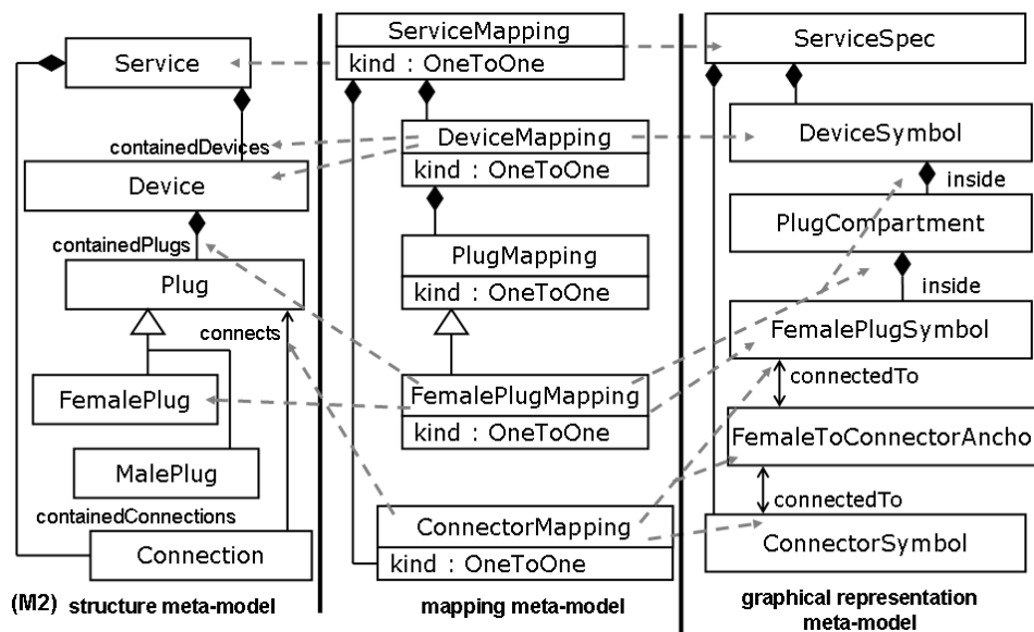
Figure 7: Illustration of mapping relationships in the Service Language
