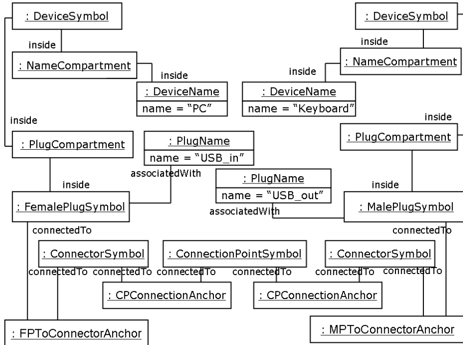
Figure 3: The diagram description model (M1) specifying a complete abstraction of the service diagram
