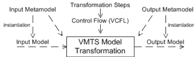
Figure 2: Principles of VMTS metamodel-based validated model transformation
