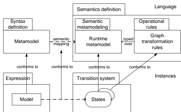
Figure 1: DMM architecture [EHHS00]
