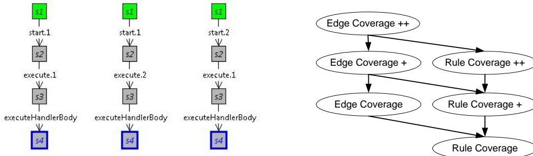
Figure 5: LTSs for the running example (ex- cerpts) Figure 6: Hierarchy of the coverage criteria [Ari11]
