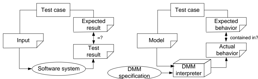
Figure 3: Testing of software systems and DMM specifications [SE09]
