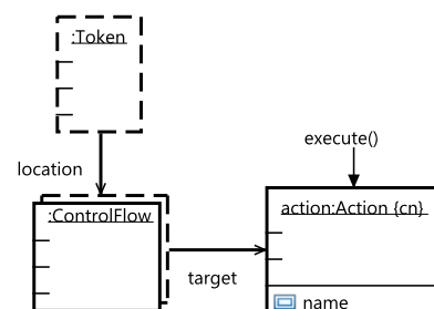
Figure 2: DMM rule action.start.1
