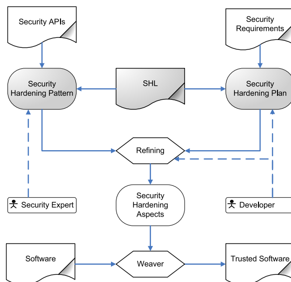
Figure 3: Framework Architecture
