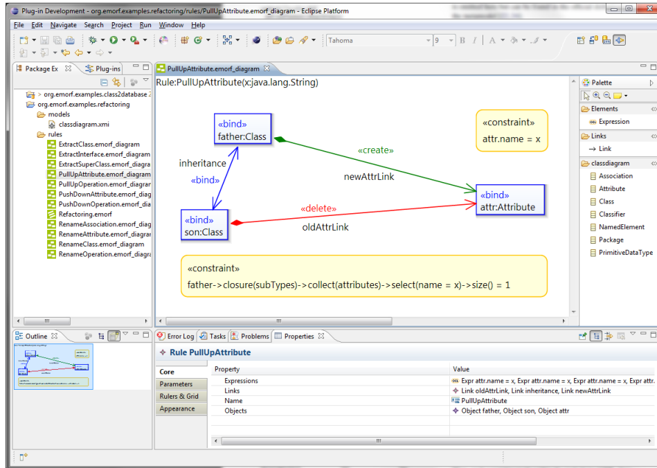
Figure 1: EMorF graphical editor showing refactoring rule PullUpAttribute
