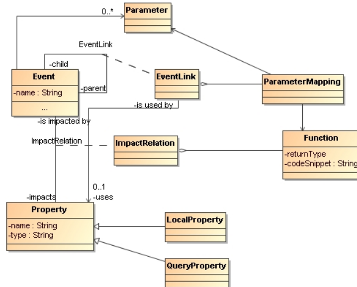
Figure 2: Behavioral Metamodel
