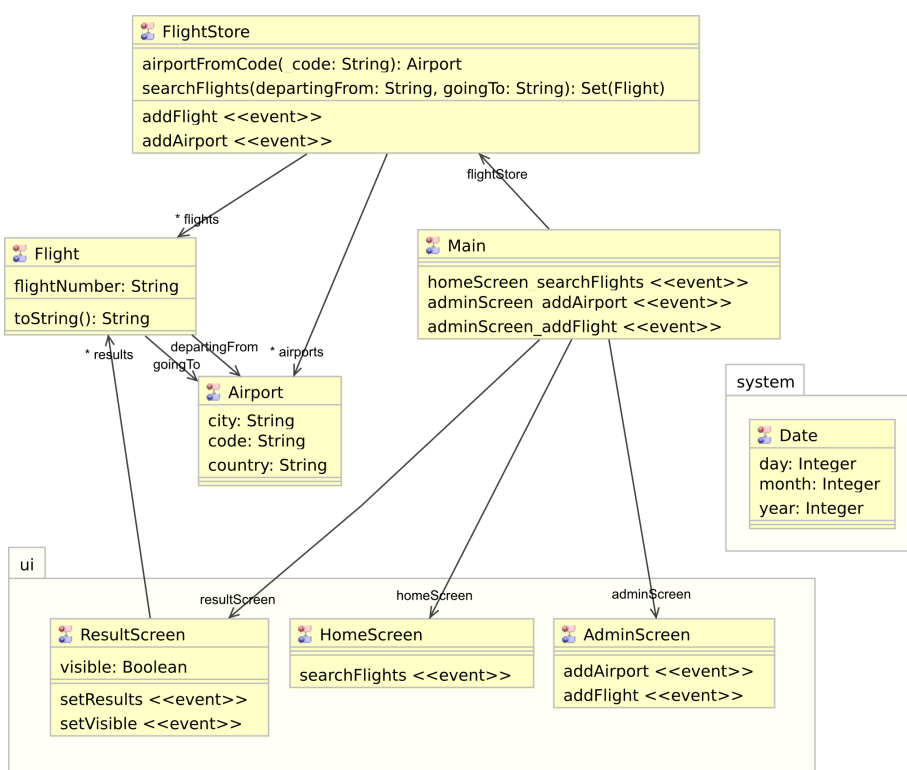
Figure 1: Class diagram of the FlightFinder application
