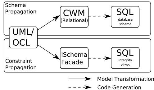
Figure 3: Mapping of UML/OCL-based domain models to relational databases
