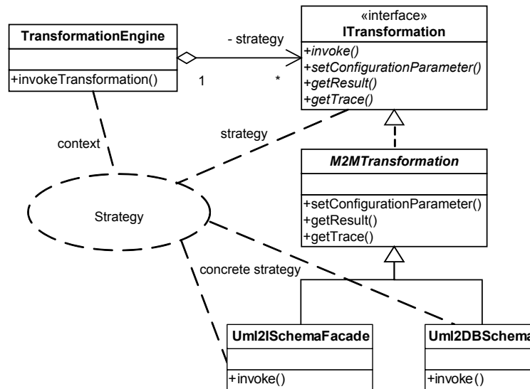
Figure 1: Architecture of the Transformation Framework
