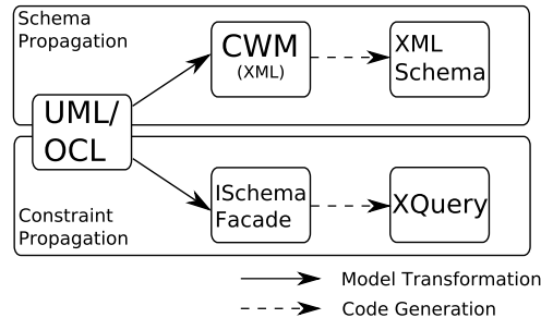
Figure 4: Mapping of UML/OCL-based domain models to XML
