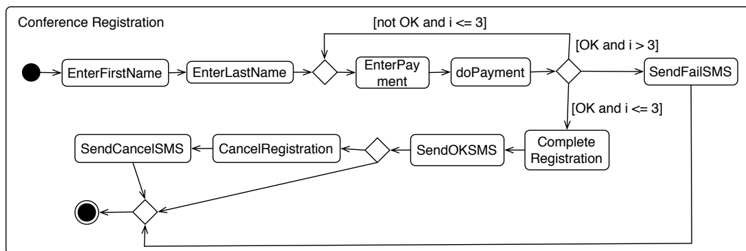
Figure 4: A Conference registration activity.
