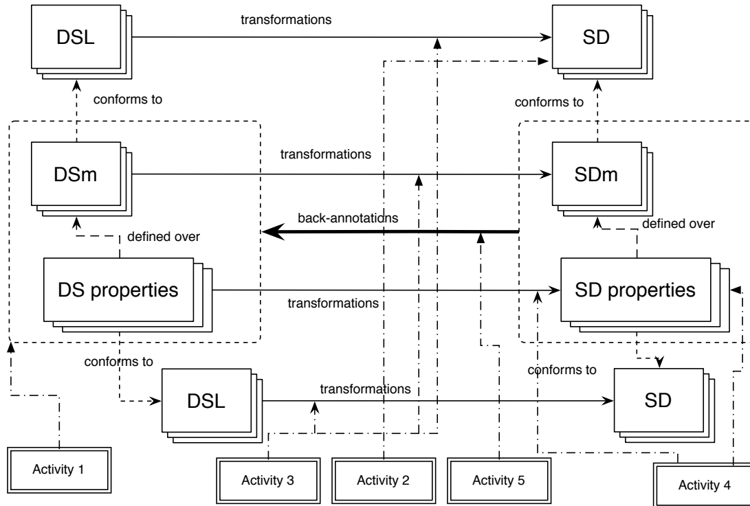
Figure 1: Framework for DSm semantics through properties.
