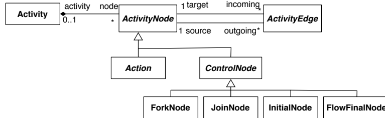
Figure 2: Small part of the UML metamodel for activity diagrams.
