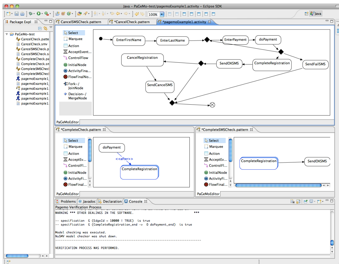
Figure 5: Screenshot of PaGeMo modelling the conference registration activity.
