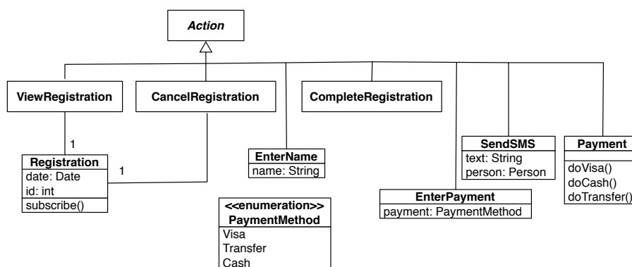
Figure 3: ConferenceRegistration metamodel.
