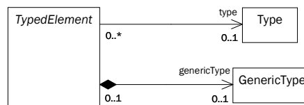
Figure 4: Typed elements and generic types
