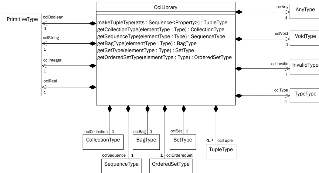
Figure 7: The facade interface for the OCL standard library types
