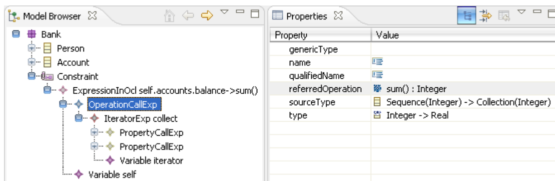
Figure 9: The abstract syntax model of the example expression
