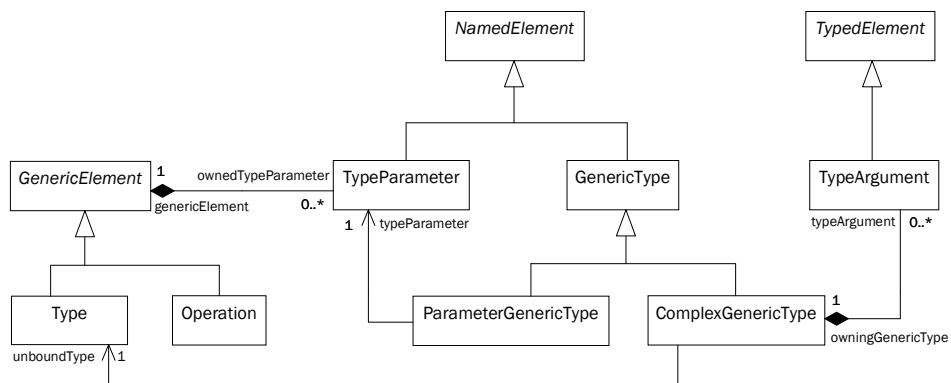
Figure 2: Generics in the pivot model
