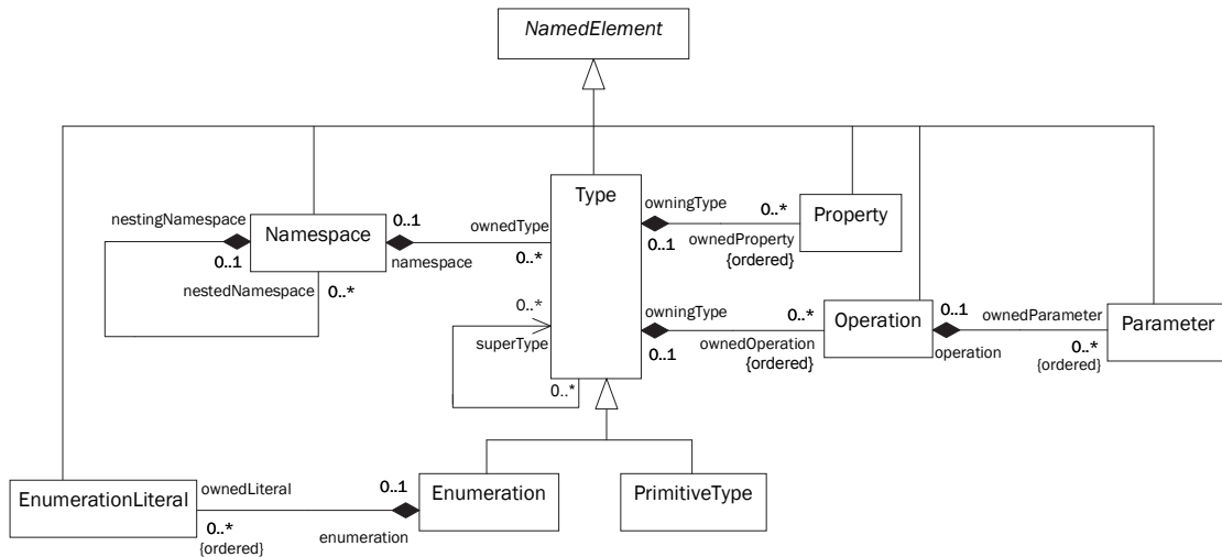
Figure 1: The main elements of the pivot model
