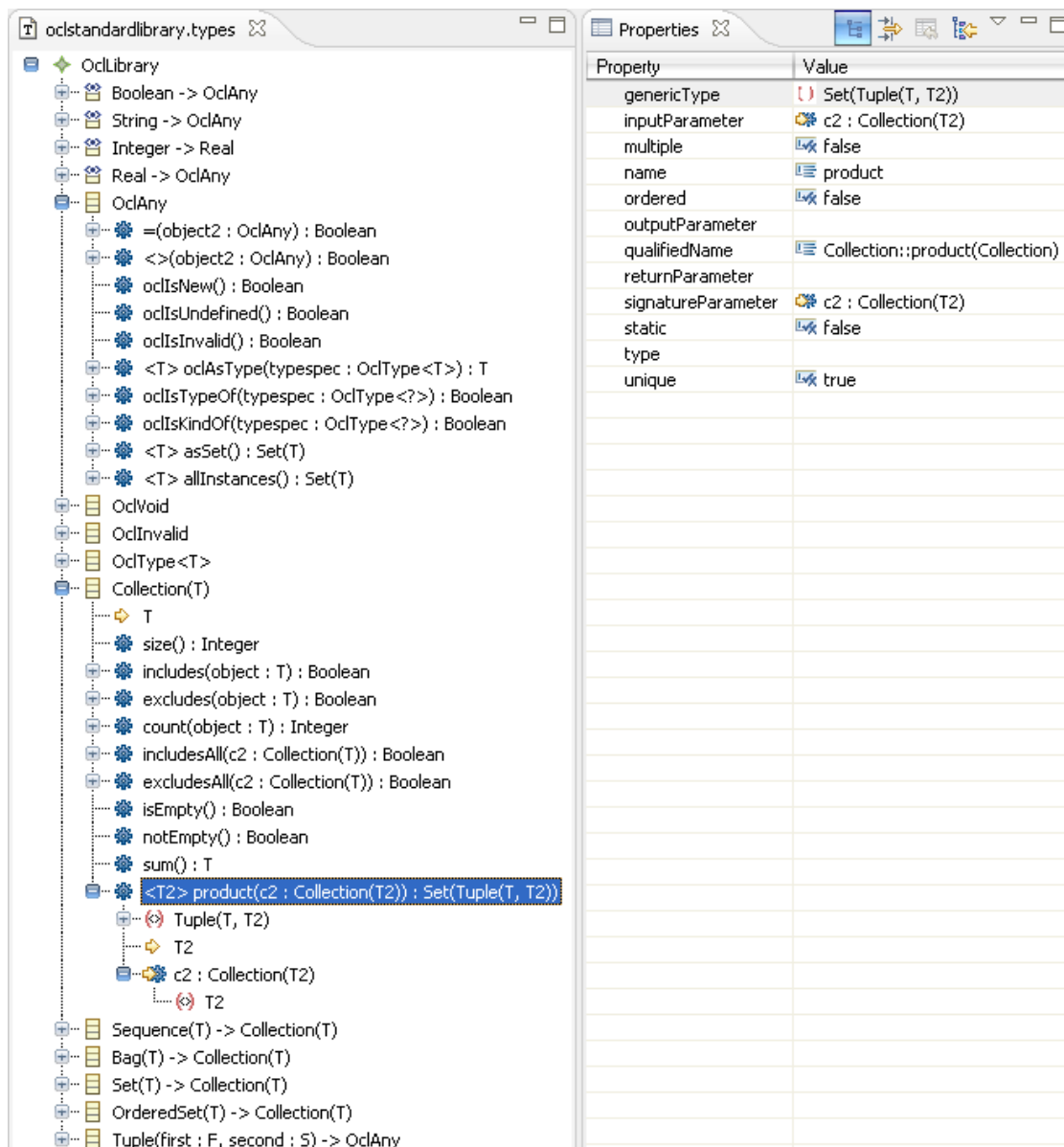
Figure 6: The model of the OCL standard library
