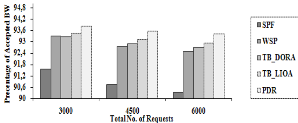
Fig. 7. The percentage of accepted BW for heavy load.
