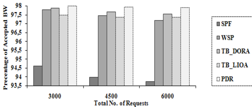
Fig. 5. The percentage of accepted BW for moderate load.
