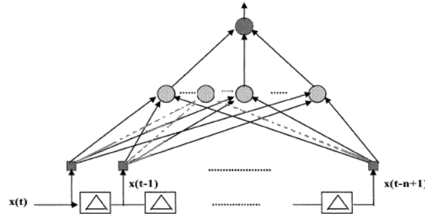
Fig. 2. Feed Forward Neural Network architecture [HDB96].
