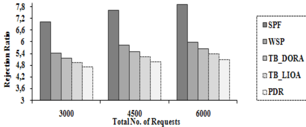
Fig. 6. The rejection ratio of requests for heavy load.
