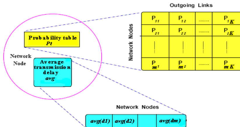
Fig. 1. The node data structures in TB algorithm [GS04].
