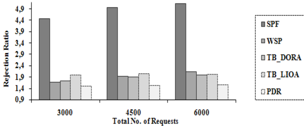
Fig. 4. The rejection ratio of requests for moderate load.
