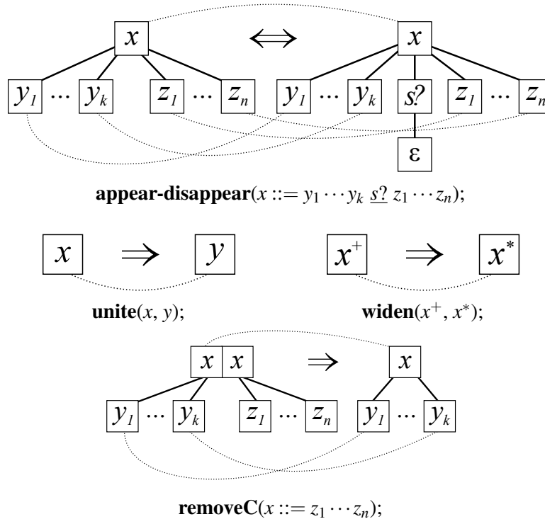
Figure 6: Graph transformations coupled to language-extending/-reducing grammar transformation operators, in the same format as used on the previous figure. appear-disappear matches the entire production rule in question but includes correspondences for each vertex so none of them can be damaged; the only modification is the addition of a new vertex with an empty value inside. unite adds all production rules of one nonterminal to another nonterminal, so all we need to do on the instance level is replace old nonterminal occurrences with the new one. widen is also unidirectional but changes only the type of one node, so the graph transformation specification looks very small. Finally, removeC removes a conjunctive clause from both the grammar and the graph defined by it. The transformation coupled to upgrade is not shown because it is identical to extract or fold which were already considered.
