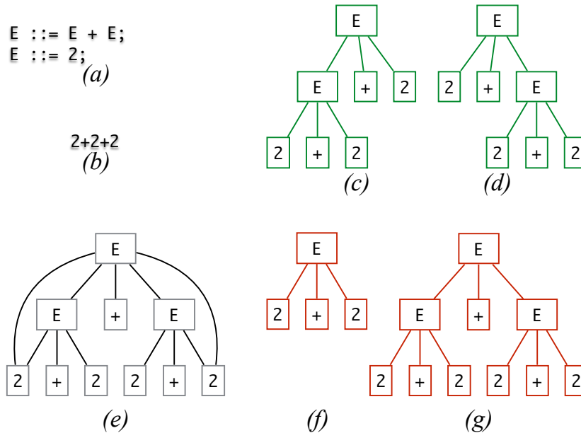
Figure 1: Demonstration that the Earley representation overapproximates parse forests: (a) a simple ambiguous grammar example; (b) a term with ambiguous parse; (c)&(d) correct parses; (e) the graph representation of the forest suggested by Earley [Ear68]; (f)&(g) incorrect parse trees that are well-formed according to the grammar (a) and covered by the parse tree representation (e), but not corresponding to the actual term (b).
