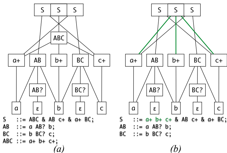
Figure 4: SPPF transformations coupled with inlining a nonterminal definition: (a) the original grammar and an SPPF of the term “abc”; (b) after applying inline (ABC). The inlining is fairly straightforward: the node in question is removed, and any previously incoming edge is replaced with the list of previously outgoing edges.
