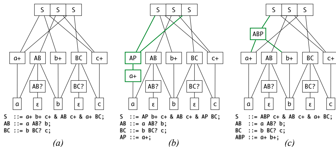
Figure 3: SPPF transformations coupled with extraction of a new nonterminal definition: (a) the original grammar and an SPPF of the term “abc”; (b) after applying extract ( AP ::= a+; ); (c) after applying extract ( ABP ::= a+ \ b+; ). The case of extracting one symbol is easier because an SPPF already has nodes for such derivations and they only need to be chained; when more than one symbol is present in the right hand side of a production rule being extracted, then a new node is introduced for all matched patterns of use.
