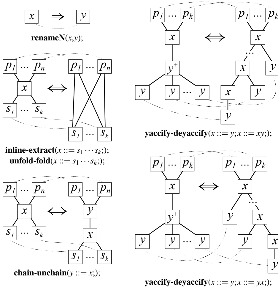
Figure 5: Graph transformations coupled to some of the language preserving grammar transformation operators: the graph on the left always represents a pattern being detected, the graph on the right defines the rewriting, dotted lines show correspondence between vertices that must not be broken by the transformation, so all incoming and outgoing edges around corresponding elements are to be preserved. renameN is very simple and intuitive: any node marked with x is replaced with a node marked with y while the node context is preserved. inline-extract shortcuts all incoming/outgoing edges to a node in question or introduces the node at their junction, depending on which direction we execute the cotransformation. unfold-fold works identically on the instance level, the differences are only observable on the grammar level. chain-unchain cuts a node in two, one of which inherits the incoming and the other one the outgoing edges. On the right, we show specifications for two ways of using yaccify-deyaccify to turn a flatter iteration-based SPPF into its deeper recursive counterpart, with left recursion variant on top and right recursion variant on the bottom. Other operators of this category from Table 1 are specified in a similar fashion.
