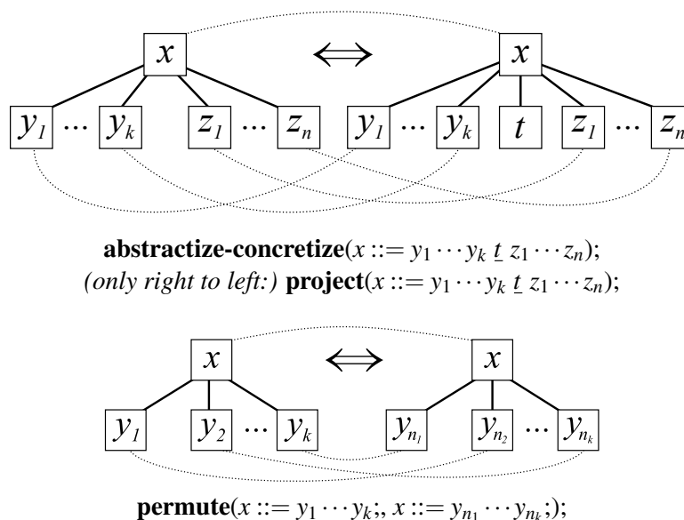
Figure 7: Graph transformations coupled to language-revising grammar transformation operators, in the same format as used on the previous figures. The transformation on top uses the same pattern that we used before for appear-disappear , which was justified back then by the empty contents of the node and now by the node in question being terminal and hence having no children. The permute operator shuffles children of one node but preserves them, which is perfectly easy expressible by the correspondence relation of the graph transformation.
