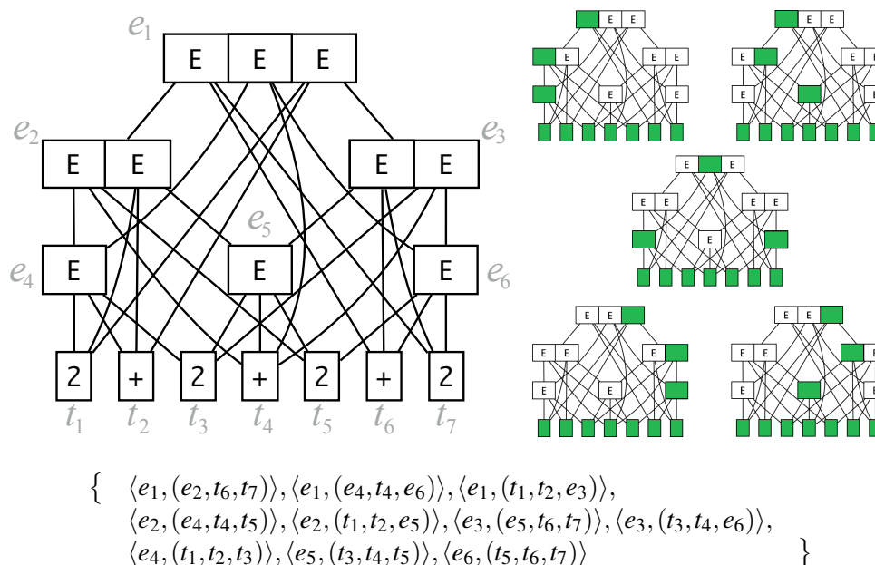
Figure 2: On the left, an SPPF graph resulted from parsing the input “2+2+2+2” with the grammar from Figure 1 (a). On the right, there are five parse trees in a forest, which are packed in a triple ambiguity, two of subgraphs of which have double ambiguities. All of them share leaves and subtrees whenever possible. Below the pictures we show its formal representation as an ordered directed graph.
