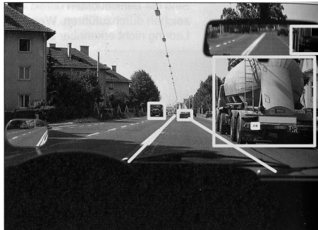
Figure 2: Relevant objects within a driving scene
