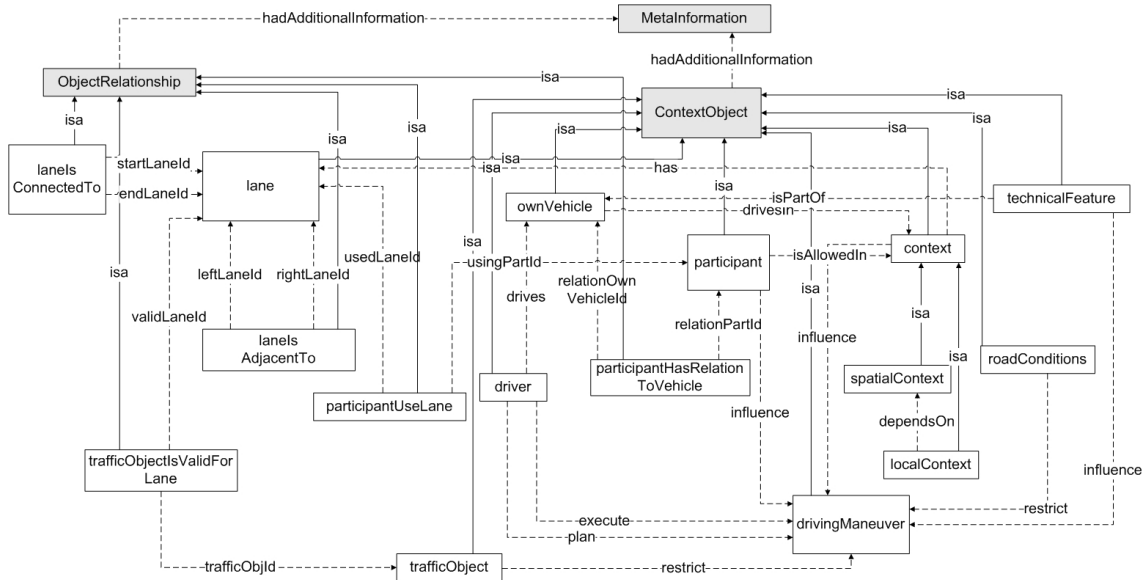
Figure 1: A context model for abstract driving scene description
