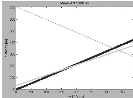
Figure 3: Speed/Distance curve of involved vehicles during overtaking
