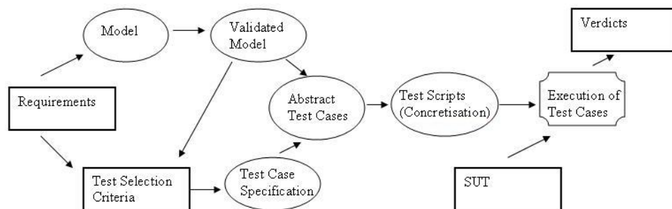
Figure 1: Model-Based Testing
