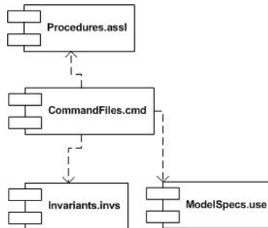
Figure 2: Deployment Diagram for USE
