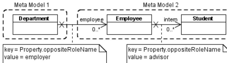
Figure 1: An example that visualizes the problem of uni-directional references
