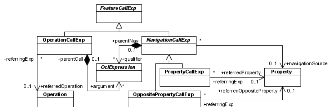
Figure 3: Extended OCL meta model
