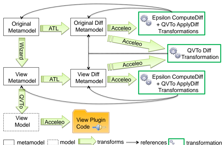
Figure 1: View Generation Process
