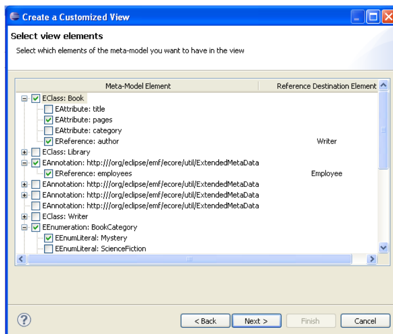
Figure 2: View Creation Wizard
