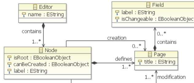
Figure 4: Editor Metamodel
