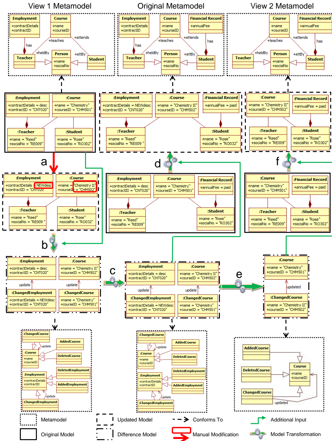
Figure 3: Synchronization
