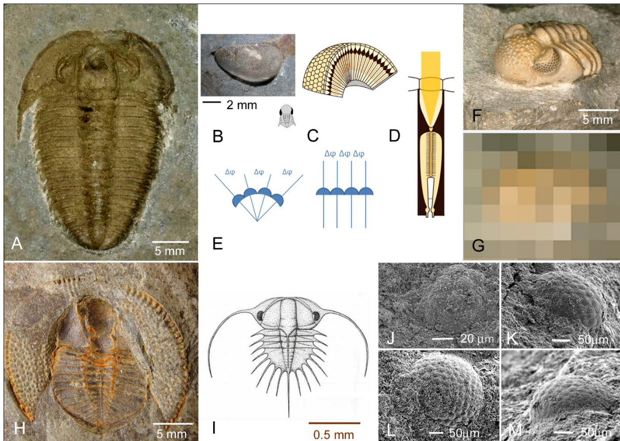
Figure 1. Trilobite compound eyes. (A) Irina oculata , Ordovician E2, Krasnojarsk, Russia, with reniform holochroal eyes. (B) Holochroal compound eye of the trilobite Pricyclopyge prisca , Ordovician, Bohemia (insert). (C) Schematic drawing of a compound eye. (D) Schematic drawing of how an apposition compound eye functions. (E) Optical axes and the fineness of scanning. (F) Phacopid trilobite Geesops schlottheimi Middle Devonian, Aueberg/Gerolstein, Germany. Note the schizochral eye with widely separated lenses. (G) E seen in an appositional-like mode with 63 facets, comparable to the specimen in E. (H) Declivolithus alfredi , Ordovician, El Kaid Errami, Morocco. Blind trilobite that lived in deep waters. (I) Ctenopyge ceciliae , tiny trilobite, Ordovician, Röstånga (Skane), Sweden. Probably the first planktonic trilobite. (J-M) Ontogenetic sequence of compound eyes of C. ceciliae .
