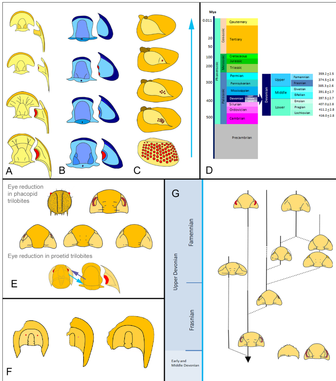
Figure 3. Eye reduction and blindness in some parallel Devonian trilobite lineages. (A) Tropicocoryphinae (Proetida), Givetian-Frasnian, with unidirectional morphological change and eye reduction. (B) Palpebralia (Proetida), Frasnian, showing progressive eye reduction. (C) Cryphops (Phacopida), base: typical phacopid eye, upwards: progressive eye reduction. (D) Geological time scale. (E) Eye shifting paedomorphically to the front in phacopid trilobites and ontogenetic change of eye position during ontogenetic development in proetid trilobites. (F) Harpes neogracilis (Harpetida), Late Frasnian, in this species eyes are reduced, while the cephalic rim enlarges to a 'compound nose' resp. 'compound ear'. (G) Eye reduction in Late Devonian lineages (comp. Feist 1995), Cyrtosymbolinae, Famennian, progressive eye reduction. (A, E-G) after Feist 1995, (B, C) after Feist 1991, (D, H) after Feist and Schindler 1994.
