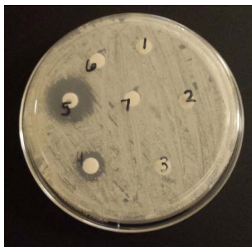
Figure 8: Kirby-Bauer disk showing antimycobacterial activity of benzoyl peroxide (4) compared to INH (5).
