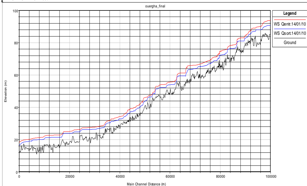
Figure 5: Resulting water profiles of the two inflow (WSQent) and outflow (WSQsort) of 14/01/2010.
