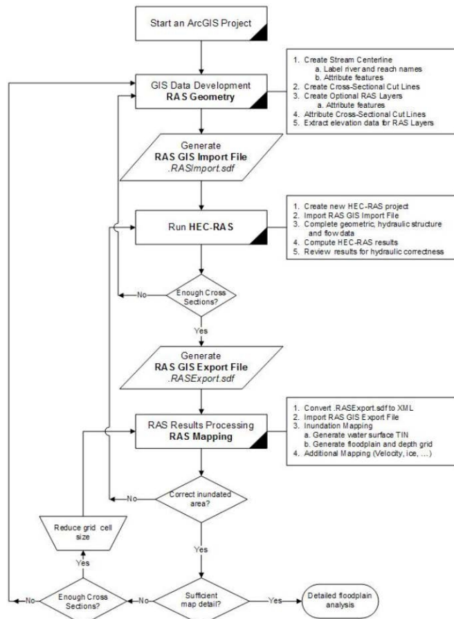
Figure 4: Diagram showing the methodology used in the modeling (Gary, 2010)
