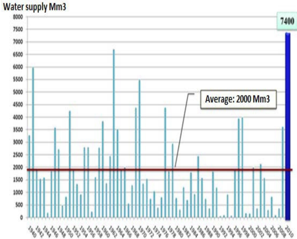
Figure 2: Ouergha river basin annual water supply on 1939-2010 (ABHS, 2006)
