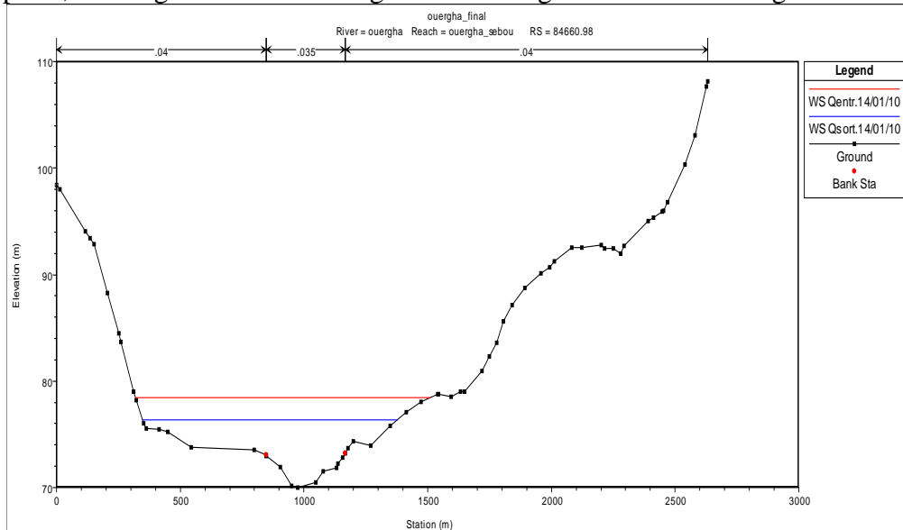
Figure 6: Resulting water levels of inflow and outflow of 14/01/2010 at the cross section 84660.98
