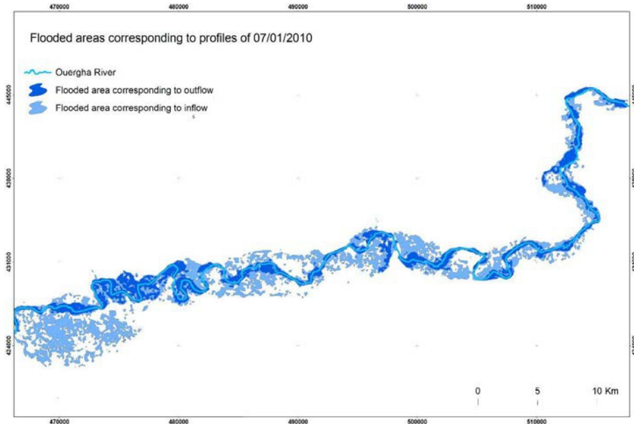
Figure 7: Flooded areas corresponding to profiles of 07/01/2010
