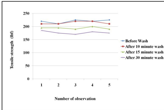
Figure 3. Graphical presentation of tensile strength (lbf) in weft way
