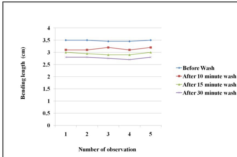
Figure 5. Graphical presentation of bending length (cm) in warp way
