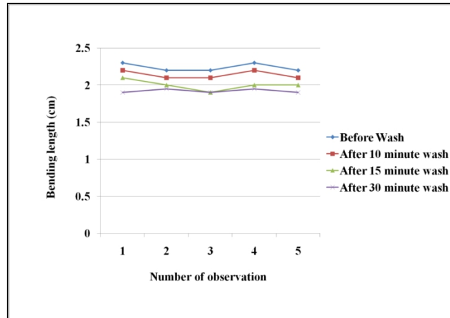
Figure 6. Graphical presentation of bending length (cm) in weft way
