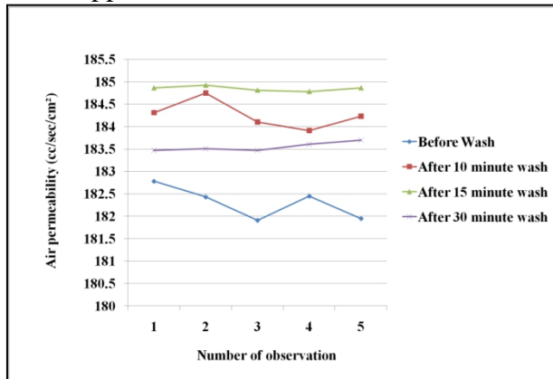
Figure 12. Graphical presentation of air permeability (cc/sec/cm 2 )
