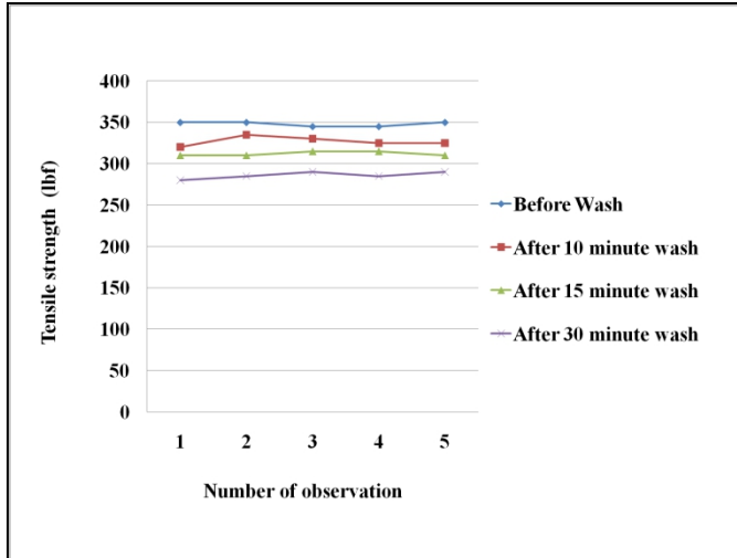
Figure 2. Graphical presentation of tensile strength (lbf) in warp way
