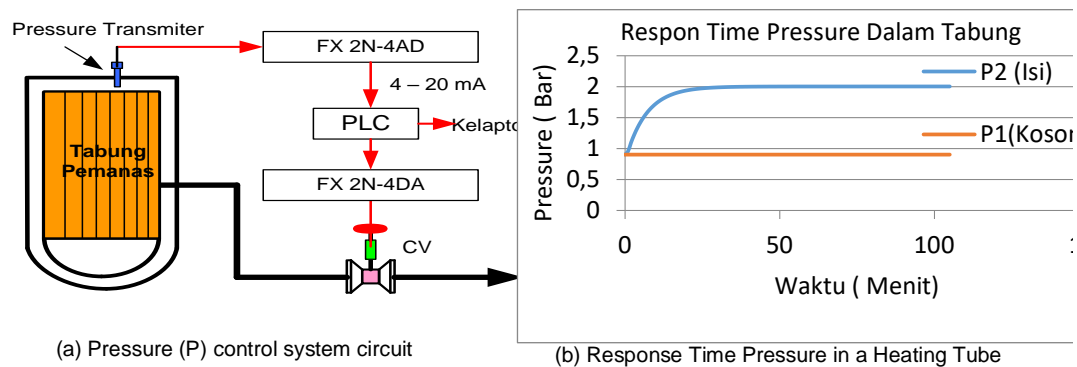
Figure 8. Pressure control system circuit and response time pressure in a heating tube
