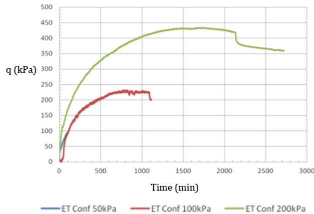
Fig. 2 Relations between Deviatoric Stress with Time
