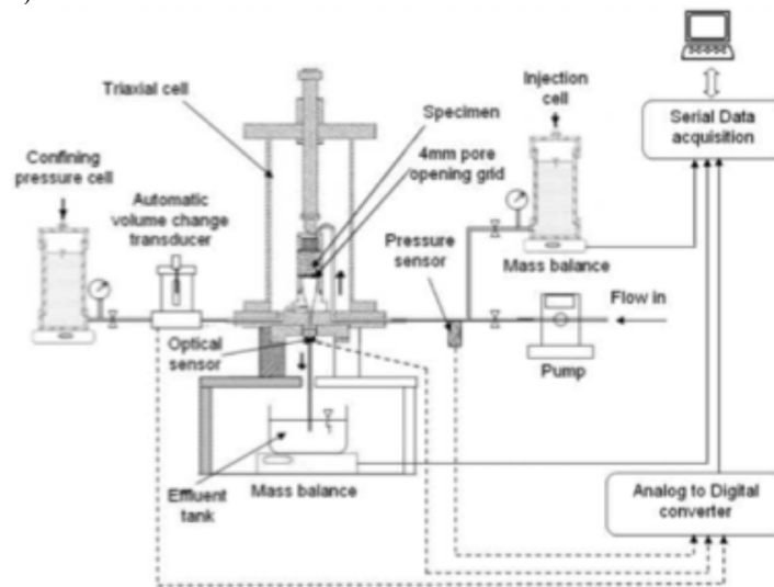
Fig 1. Schematic Diagram of Triaxial Erodimetre
