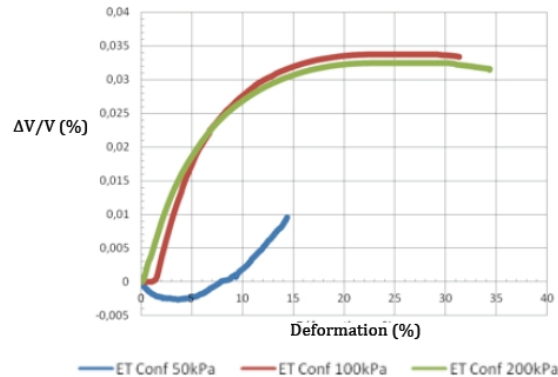
Fig. 4 Variation volumic in function of deformation
