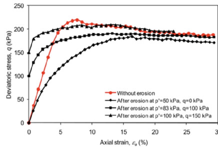
Fig. 6 Deviatoric stress in function of deformation from Chang&Zhang (2011)
