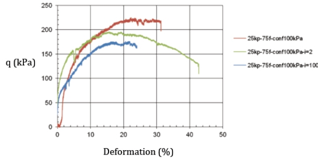
Fig. 5 Comparison of deviatoric stress in function of deformation before erosion and after erosion
