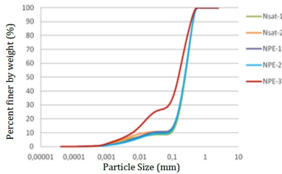
Fig. 7 Grain Size Distribution of eroded particle with gradient hydraulic=2
