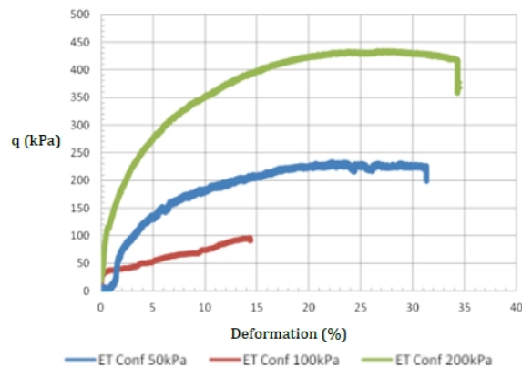
Fig. 3 Deviatoric Stress in function of deformation
