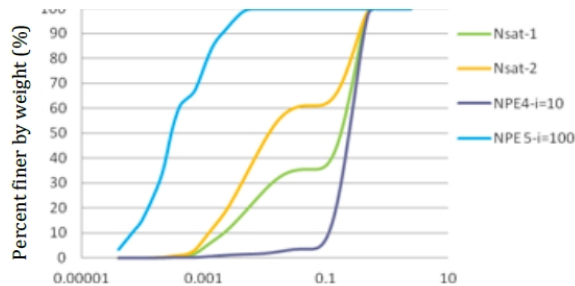
Fig. 8 Grain Size Distribution of eroded particle with gradient hydraulic=10-100
