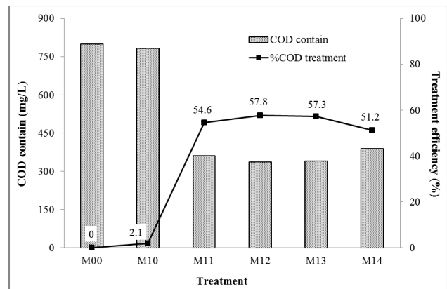
Figure 1. COD treatment efficiency vs PAC quantity
