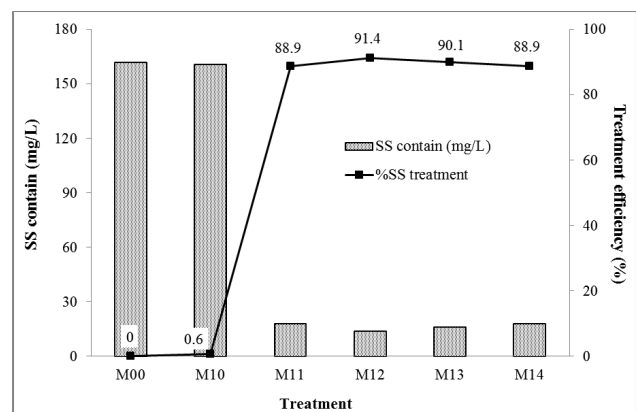
Figure 3. SS treatment efficiency vs PAC quantity
