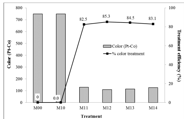
Figure 2. Color treatment efficiency vs PAC quantity
