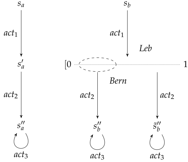
Figure 4.4: It holds s_a \simeq^{sou} s_b but neither s_a \leq^{tr} s_b nor s_a =^{tr} s_b .
