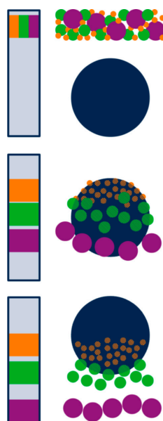
Figure 8. Separation principle of size exclusion chromatography showing the packed column (left) and one selected bead (right) during injection (top), separation (middle), and elution (bottom) of a three-component mixture. Proteins are separated according to decreasing size due to a reduction in available pore volume for larger molecules. Adapted from [128], reproduced with permission from John Wiley and Sons, 2011.
