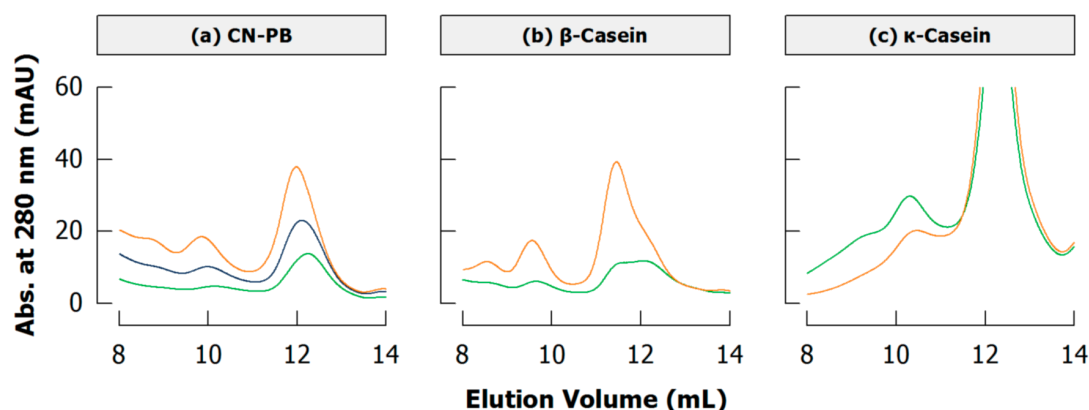
Figure 11. Sections of typical size exclusion chromatograms (Superdex 200 column) of cross-linked (a) casein in phosphate buffer (CN-PB); (b) \beta -casein; and (c) \kappa -casein depicting monomers ( \sim 12 mL) and dimers ( \sim 10 mL) (originally presented in [94]; see also Appendix A.4). Samples were incubated with transglutaminase for 1 (orange), 2 (blue), or 3 h (green) (see Appendix A.1 for experimental details).
