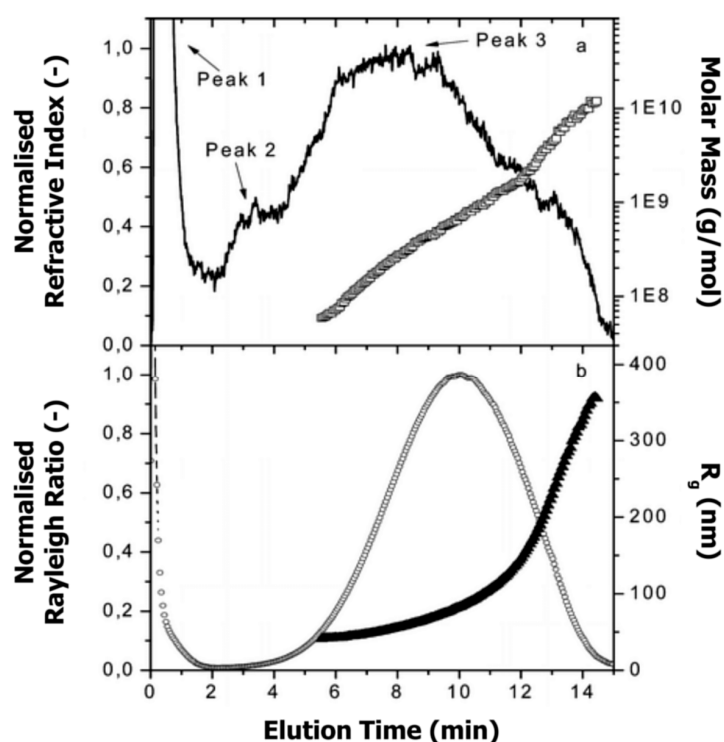
Figure 14. (a) Molar mass ( \square ) and normalised refractive index signal (-) vs. elution time, and (b) radius of gyration ( R_g ; \blacktriangle ) and normalised Rayleigh ratio ( 90^\circ scattering angle; \circ ) vs. elution time for casein micelles in milk. Reproduced with permission from [188]. Copyright by American Chemical Society, 2000.
