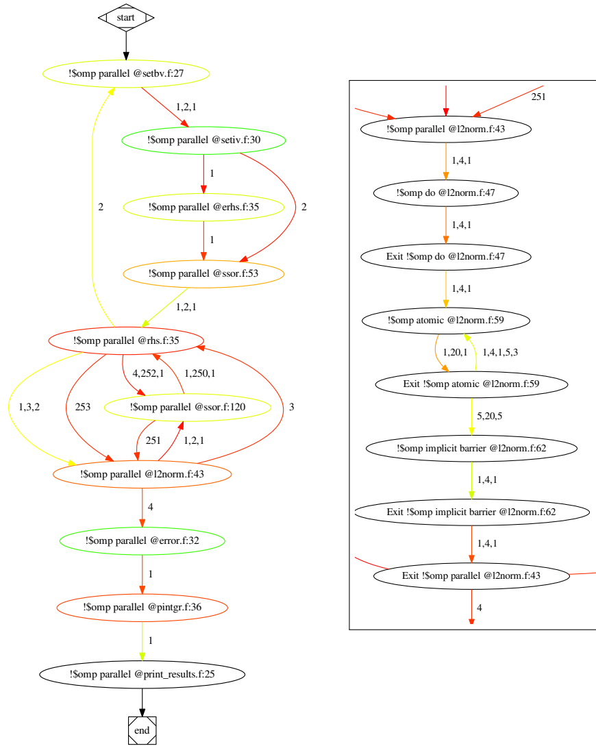
(a) Master Thread, Event flow graph of parallel regions (b) Event flow graph of OpenMP instrumentation, zoom into parallel region @l2norm.f:43
