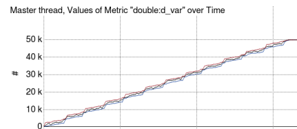
(b) OMP_SCHEDULE=dynamic,4096
