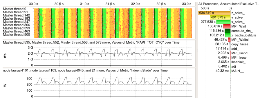
Fig. 9: MPI parallel NPB BT (576 ranks). Left side (from top to bottom): Executed functions (function names on right panel), average frequency of involved processor cores, average power consumption of nodes.
