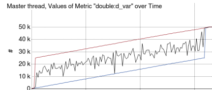
(a) OMP_SCHEDULE=static
