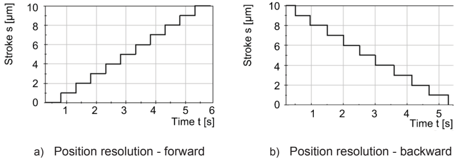
Figure 6: Step response of hydraulic linear drive controlled with proportional and digital valve
