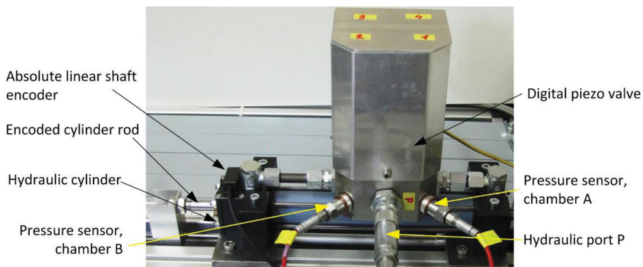
Figure 2: Real picture of prototype linear drive controlled with digital piezo valve
