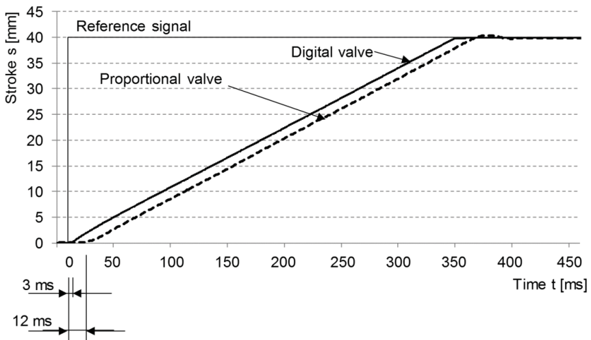
Figure 6: Step response of hydraulic linear drive controlled with proportional and digital valve
