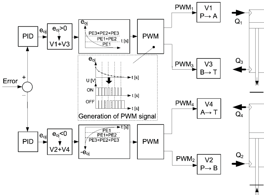
Figure 3: Block diagram of control method
