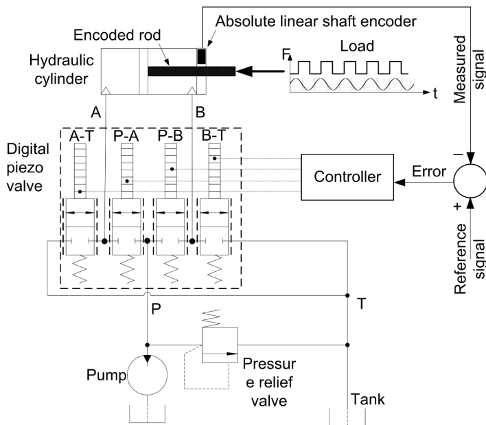
Figure 1: Scheme of hydraulic linear drive controlled with digital piezo valve
