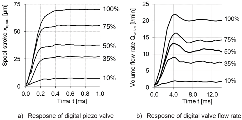
Figure 4: Characteristics of digital piezo valve
