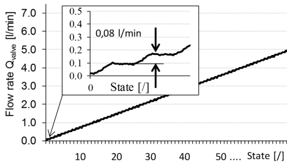
Figure 5: Flow rate characteristics of on/off piezo valve and the step size (state P→A)
