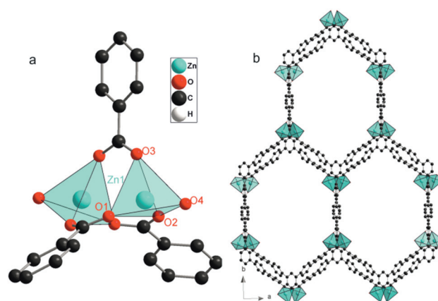
Fig. 1 SBU unit of DUT-40 (a) and the crystal structure along the c axis (b).
