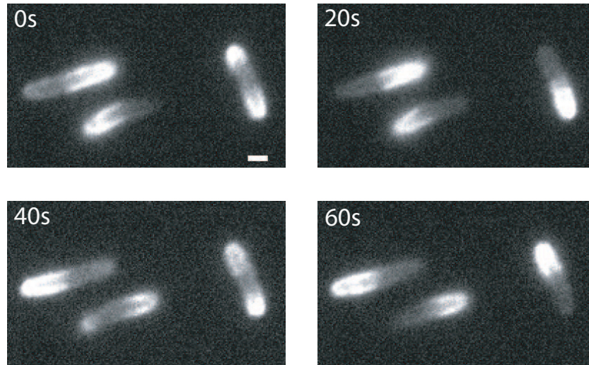
Figure 2.1: Oscillations of GFP-MinD in E. coli . Fluorescence images of GFP-MinD in three cell at subsequent time points separated by 20s. Scale bar: 1 \mu m.
