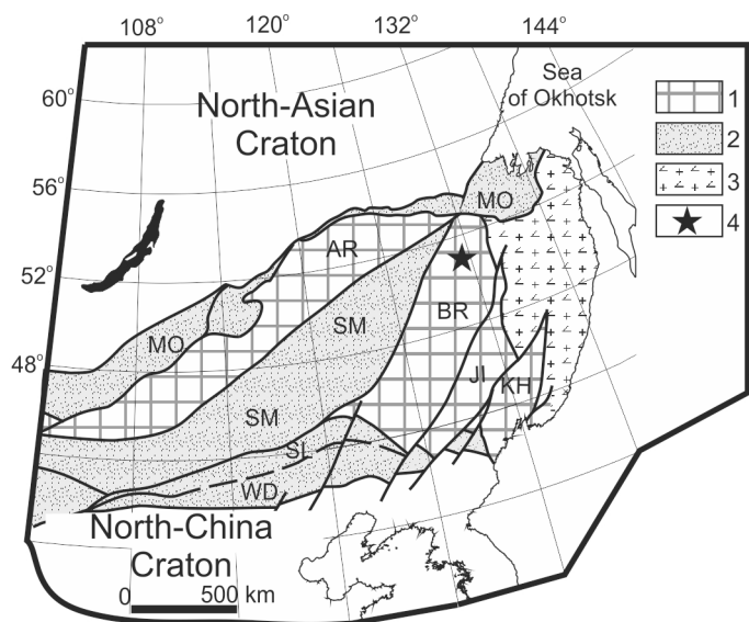
Fig. 1. Generalized structural scheme of the Eastern part of the Central Asian orogenic belt (modified from [Parfenov et al., 2003]).
