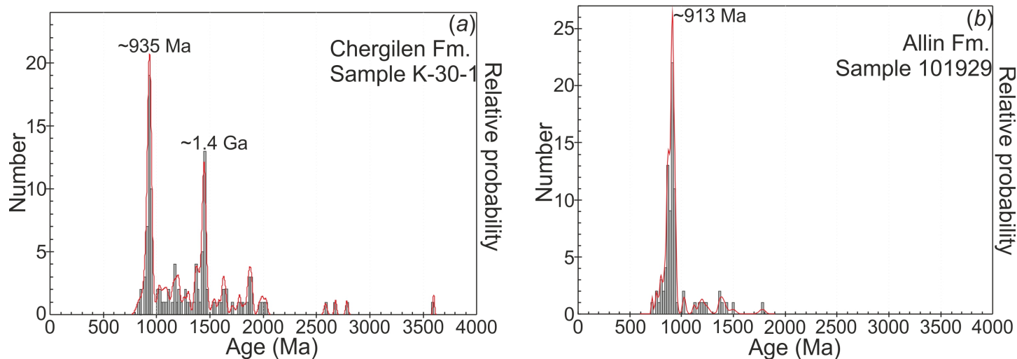
Fig. 2. Histograms and relative probability plots of ages of detrital zircons from siltstone of the: a – Chergilen Formation (sample K-30-1) and b – siltstone of the Allin Formation (sample 101929).
