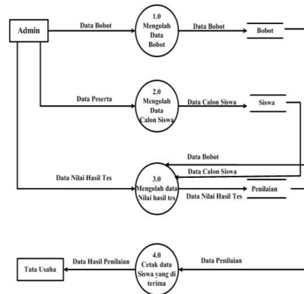
Gambar 6. DFD level 0
