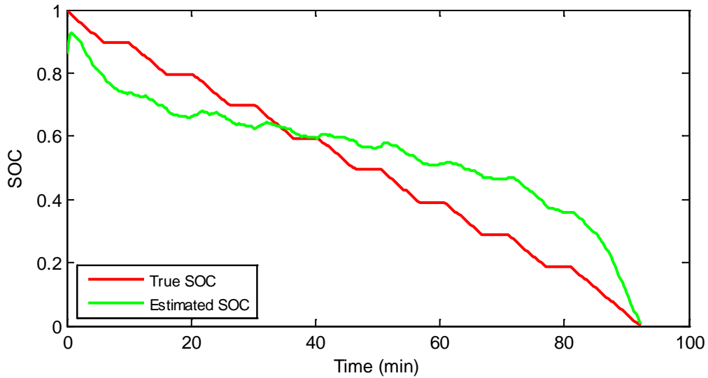
(b) Unnewehr model (discharge)
