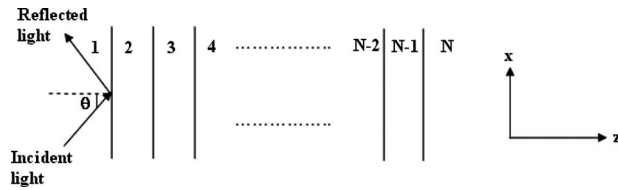
Fig. 6 Basic N -layer system to describe the transfer matrix method.
