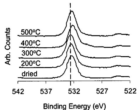
FIG. 9. O 1s XPS spectra of sol-gel silica films containing 1 mol % Ag after different heat-treatments.
