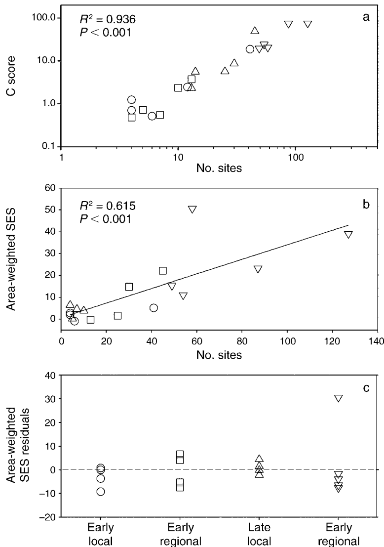
FIG. 1. The effect of study scale (number of study sites) significantly affected (a) computed C scores (note log–log scale) and (b) area-weighted standard effect scores (SES). Residuals of the sites vs. area-weighted SES regression (reorganized per temporal/spatial class in panel c) were used as additional weights in species co-occurrence analyses. See Appendix B for details.
