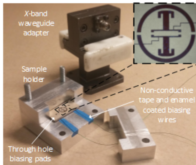
Figure 3.19: Measurement setup showing the fabricated dual-resonant unit cell with biasing wires, sample holder, and the waveguide adapter
