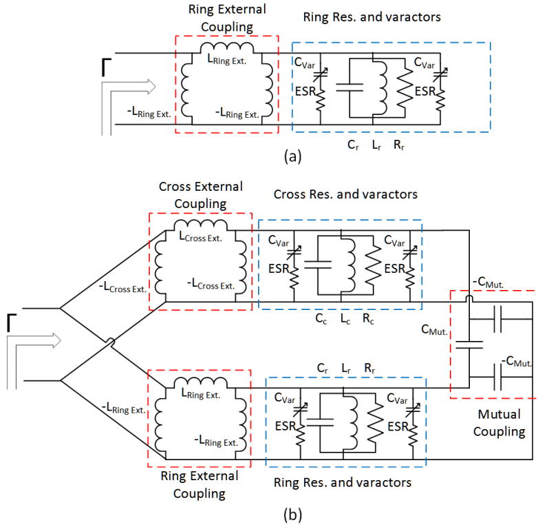
Figure 3.2: Equivalent circuit model for (a) isolated ring and (b) dual-resonant unit cell configurations.
